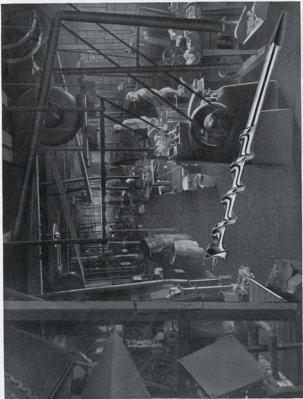
Partial View of Forging Room
